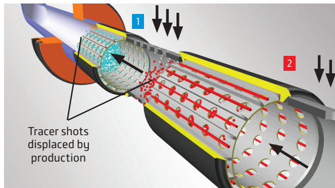
Fig. 3 - Initial production from the zones displaces the tracer shots 1 and 2 to surface. The arrival time of each is dependent on the inflow upstream of each tracer location.
