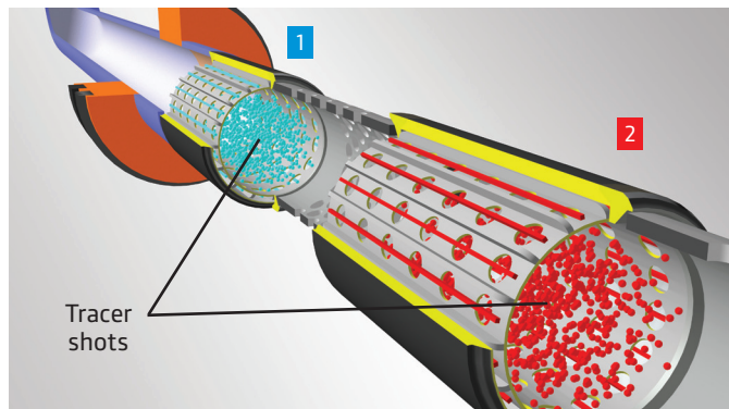
Fig. 2 - During a shut-in, the intelligent tracers in each zone (zone 1 blue, zone 2 red) release their unique molecule signature into the fluids inside the tubing, creating tracer shots.
