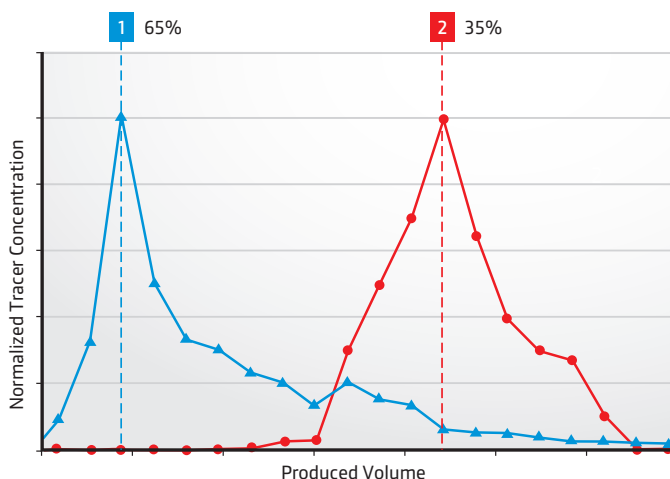
Fig. 4 - Arrival Time model best simulation fit between predicted (dashed lines) and actual arrivals (peaks). The resulting inflow distribution for each zone is shown on the right.
